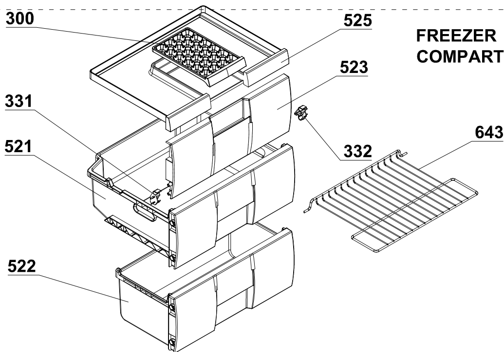
REFRIGERATOR COMPARTMENT
