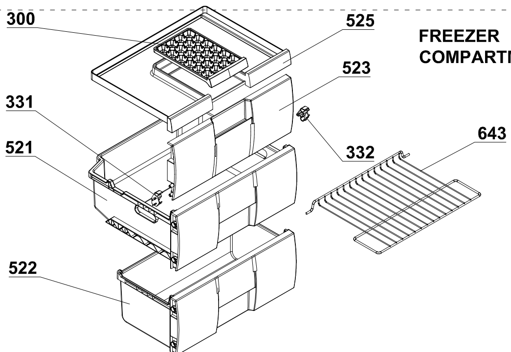
REFRIGERATOR COMPARTMENT
