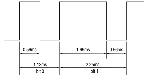
Fig 5-2 BIT STRUCTURE
