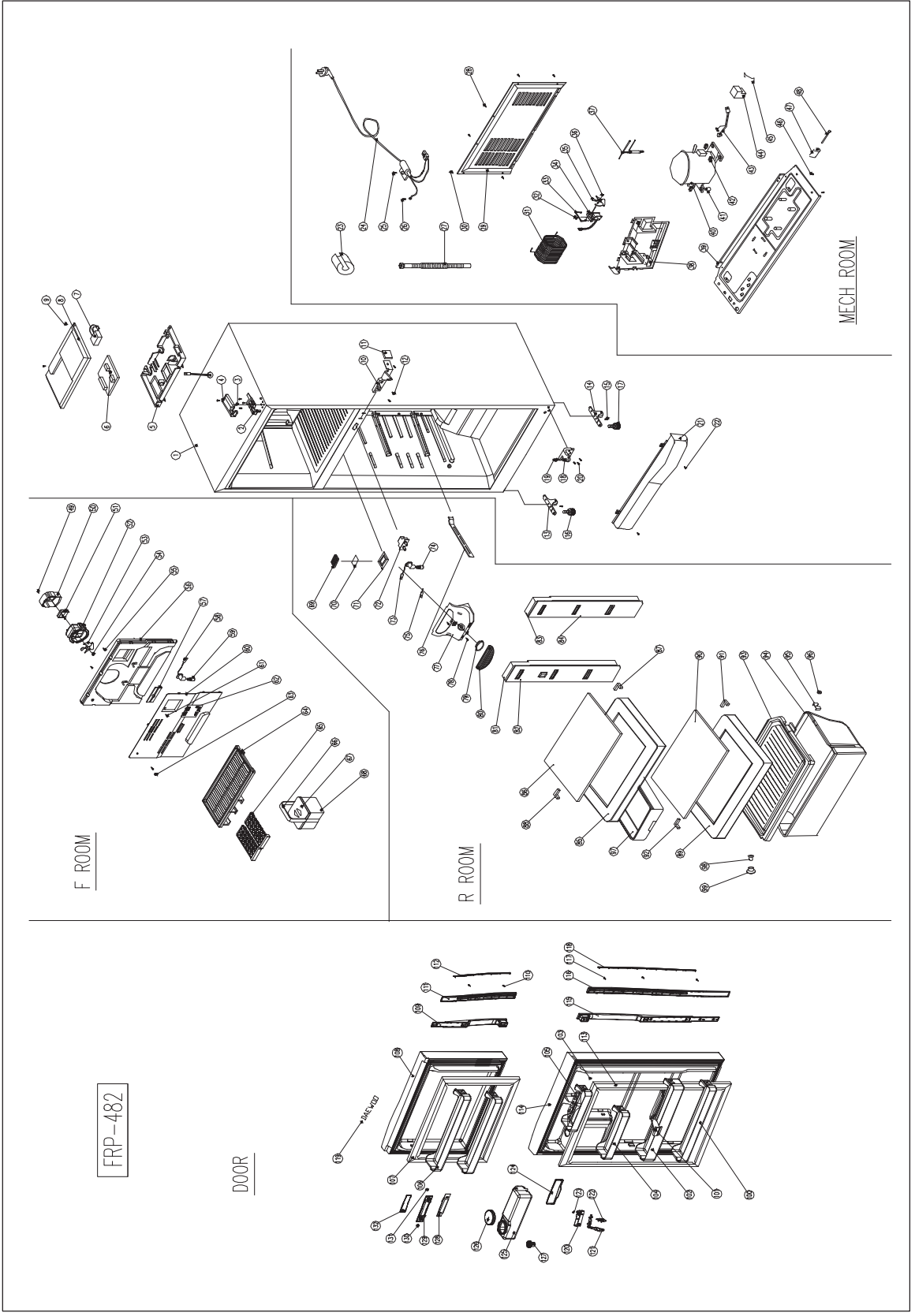
6-2. FR-590NW TOTAL EXPLODED VIEW
