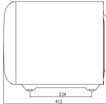
Fig.2 Side view
