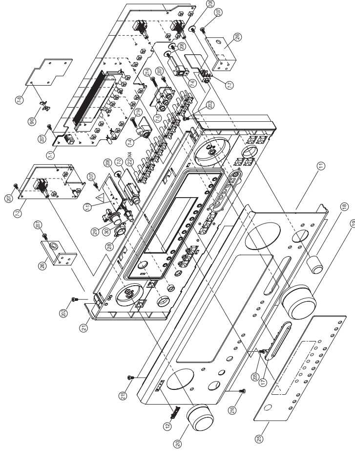
AVR-888 E3 Model : FRONT PANEL EXPLODED VIEW
