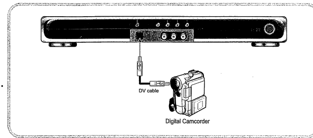
<DVR-80PT/DVR-160PT/DVR-250PT>
