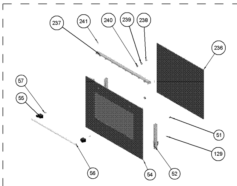
FLAT OVEN DOOR WITH FULL GLASS STRUCTURE (OPTIONAL)
