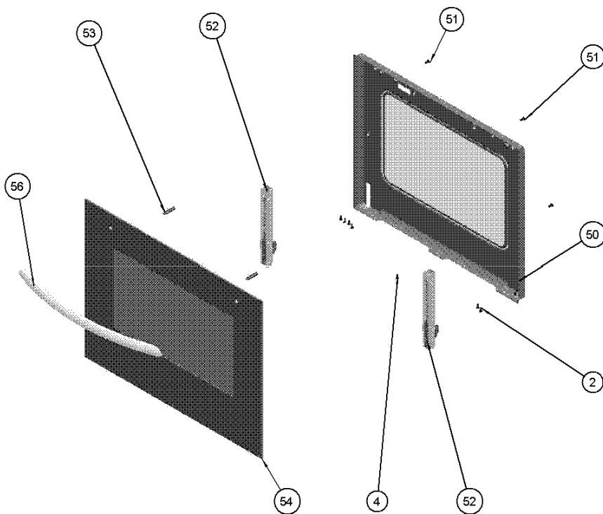
FLAT OVEN DOOR WITH INNER METAL FRAME
