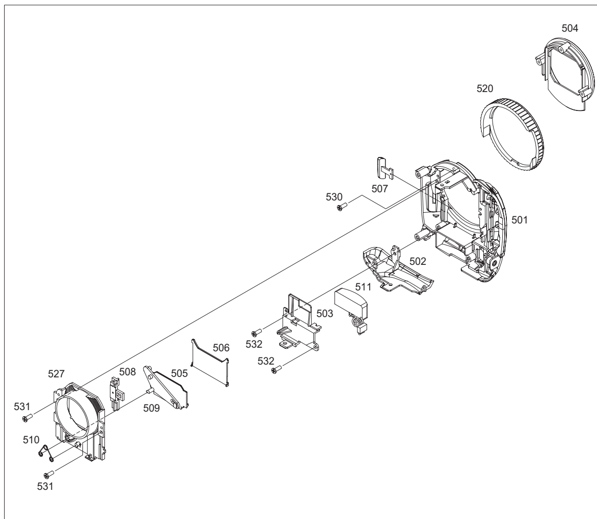
FRONT ASSEMBLY
