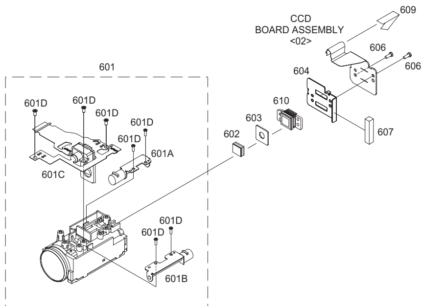
FRONT ASSEMBLY
