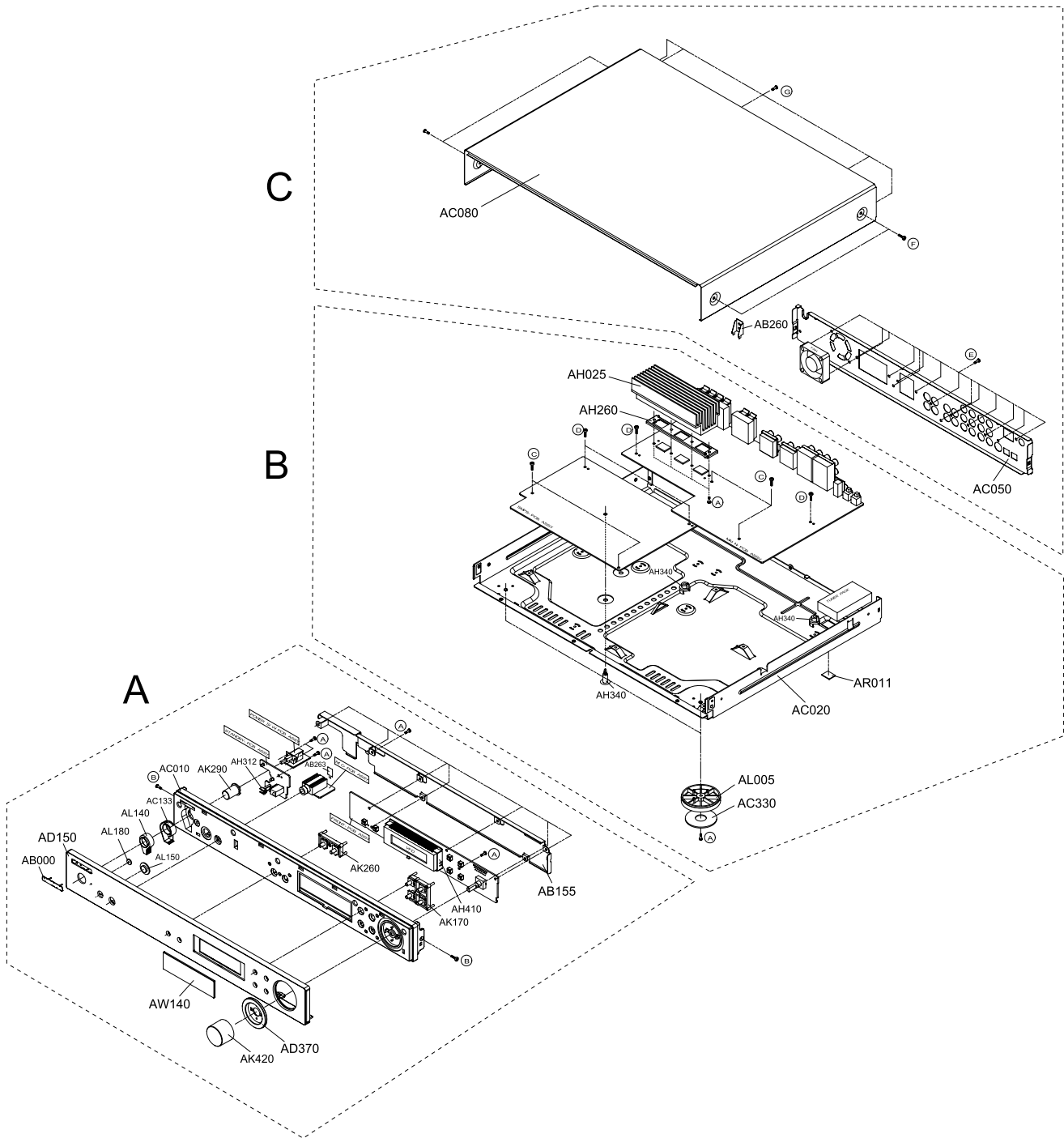
AV-R600 EXPLODED-VIEW DRAWING
