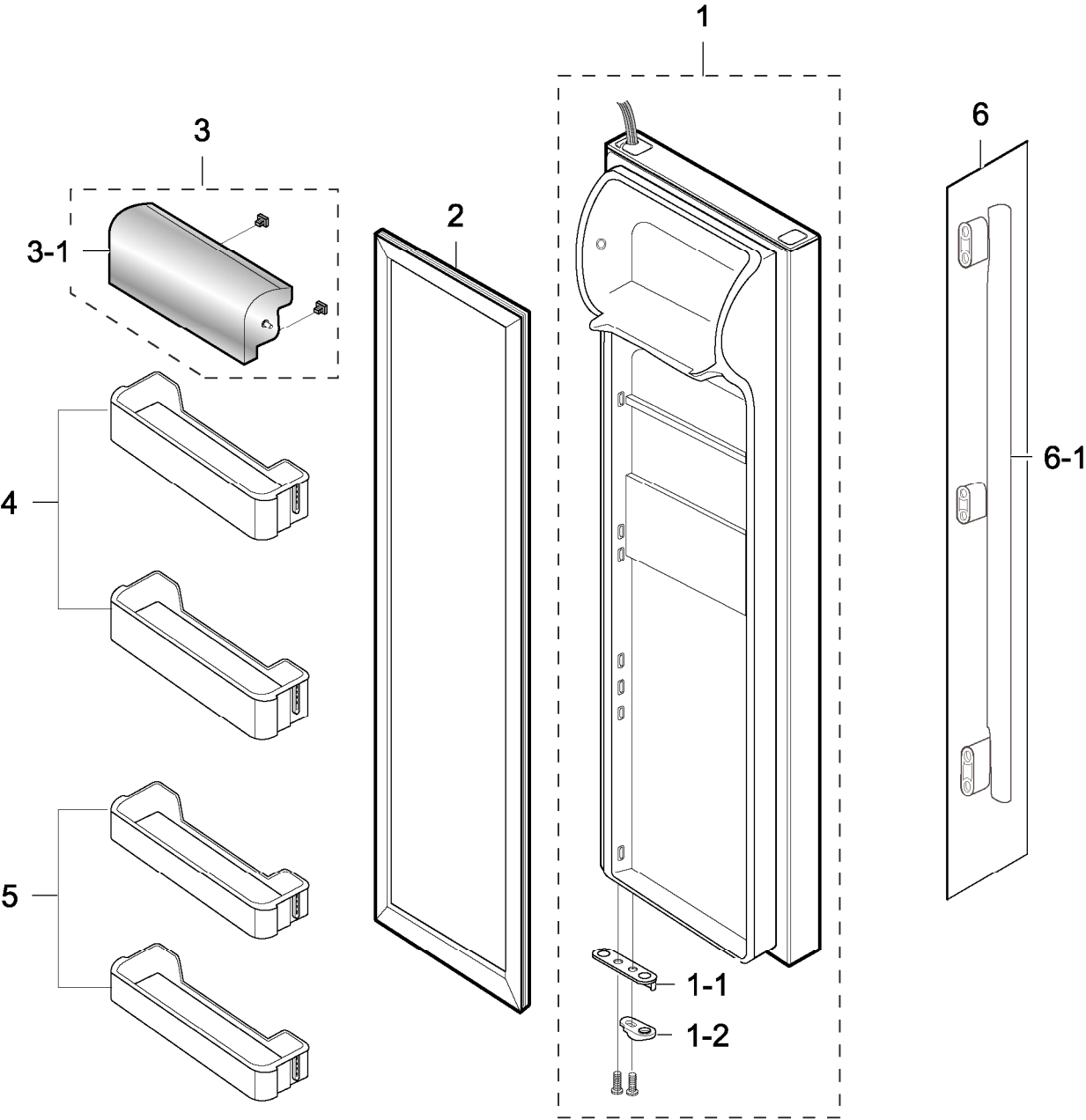
Exploded View
