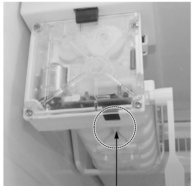
Thermistor(Ice-Maker)
