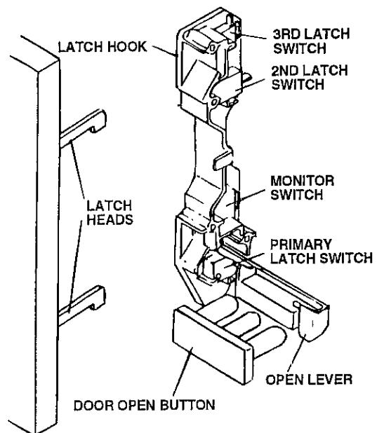
Figure C-5 Latch Switches Adjustment
