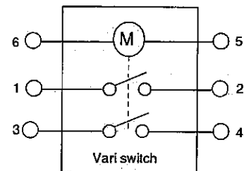
Timer motor with vari switch
