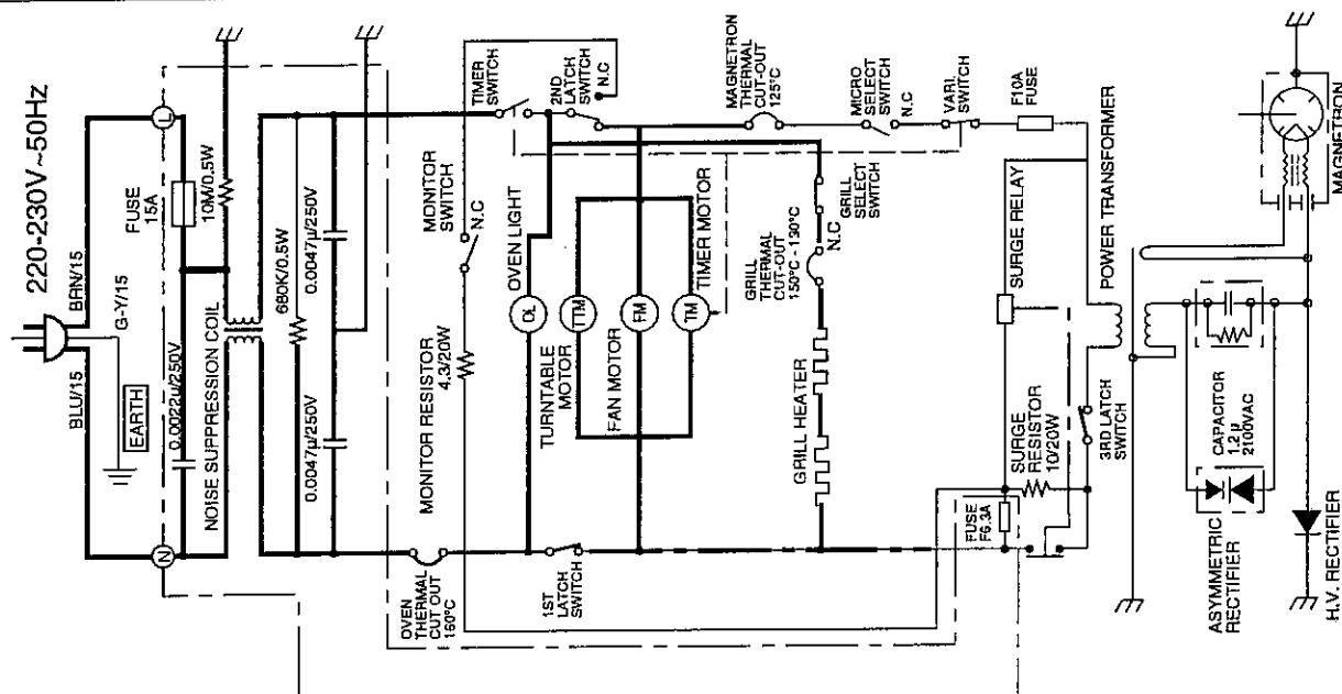
Figure O-3 Oven Schematic-Grill Cooking Condition
