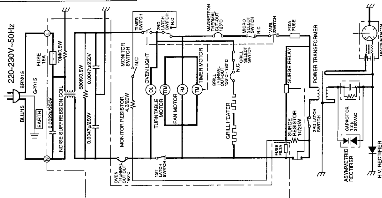
Figure O-4 Oven Schematic-Dual Cooking Condition
