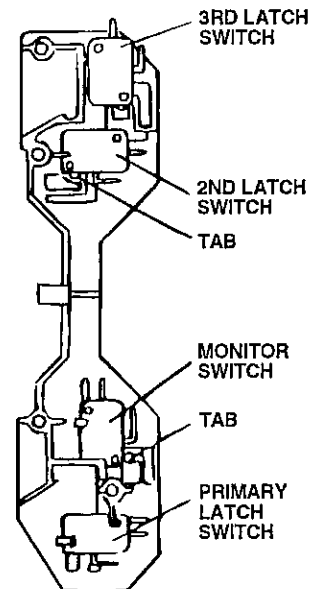
Figure C-4. Switches
