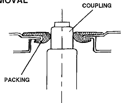
Figure C-1. Turntable Coupling
