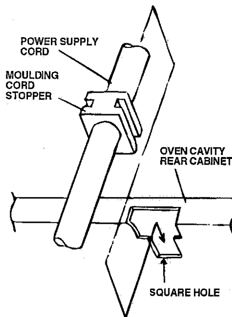
Figure C-3 (b) Replacement of Power Supply Cord
