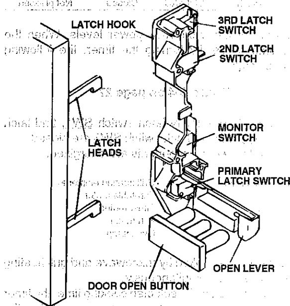
Figure D-1. Door Open Mechanism
