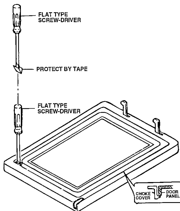
Figure C-7. Choke Cover Removal
