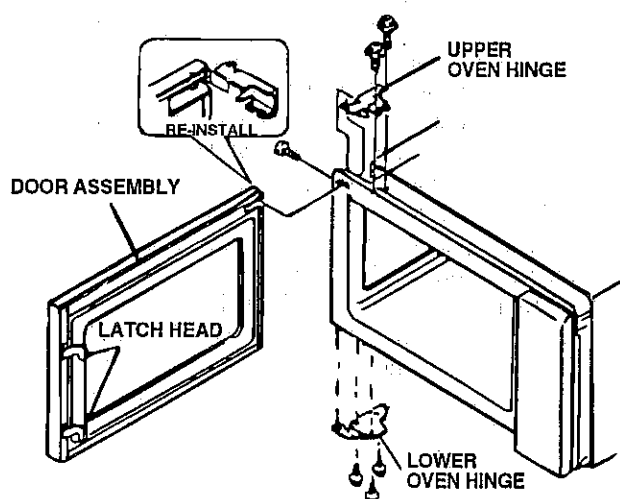
Figure C-6. Door Assembly Replacement and Adjustment
