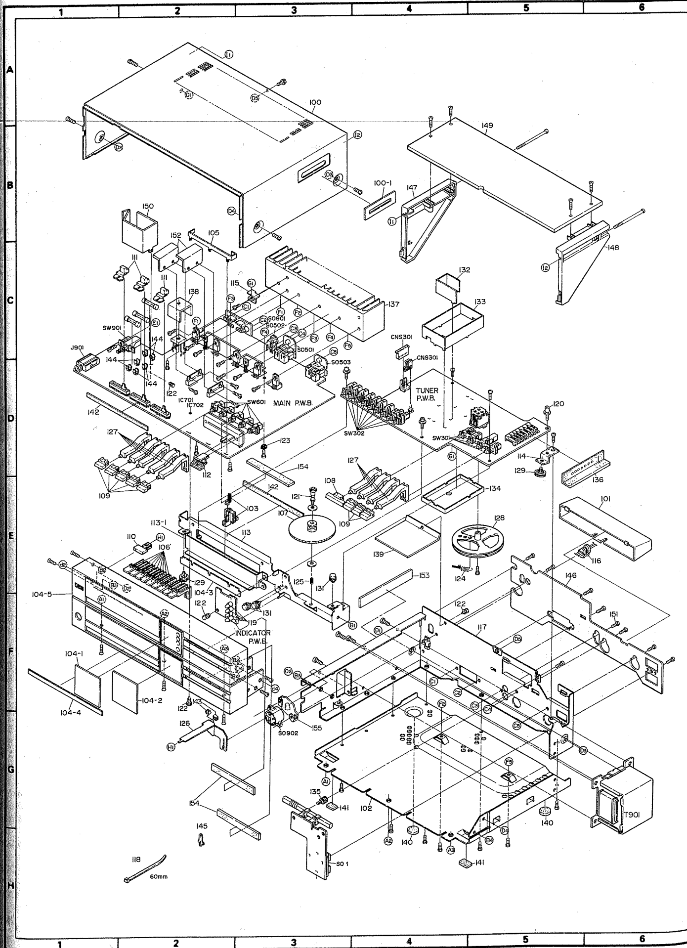
Figure 27 CABINET EXPLODED VIEW
