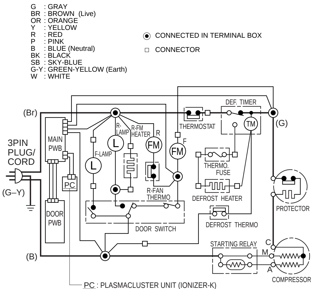
Figure W-1. Wiring Diagram (SJ-PK60M,PK65M,PK70M)
