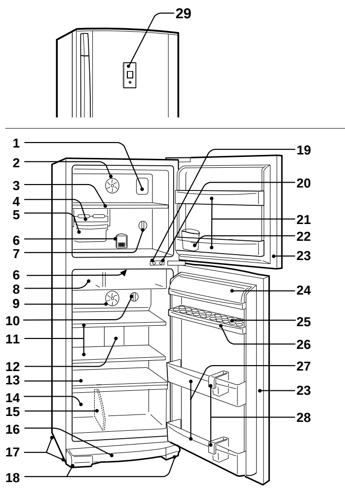
Figure D-1. External Description
