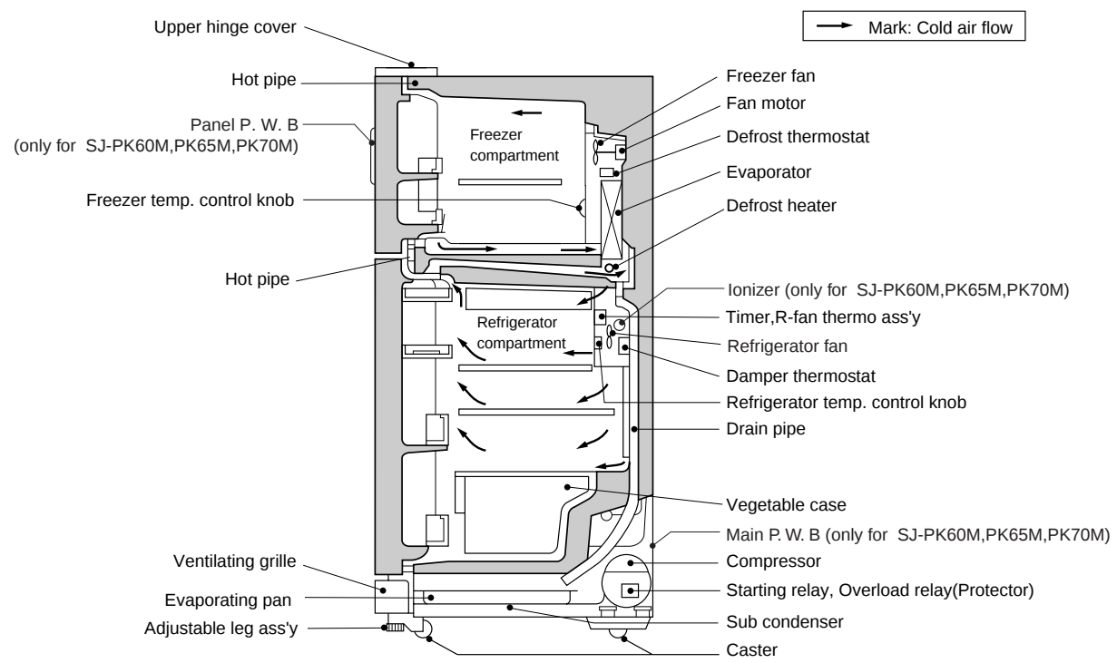
Figure D-2. Constructions
